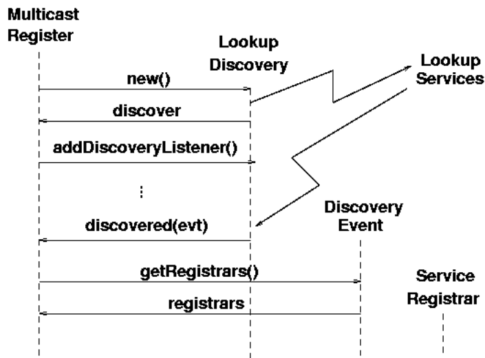
Figure 4-2. UML sequence diagram for discovery
