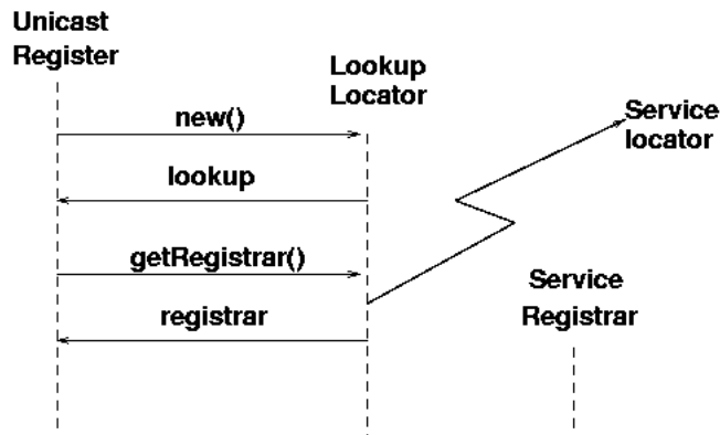
Figure 4-1. UML sequence diagram for lookup
